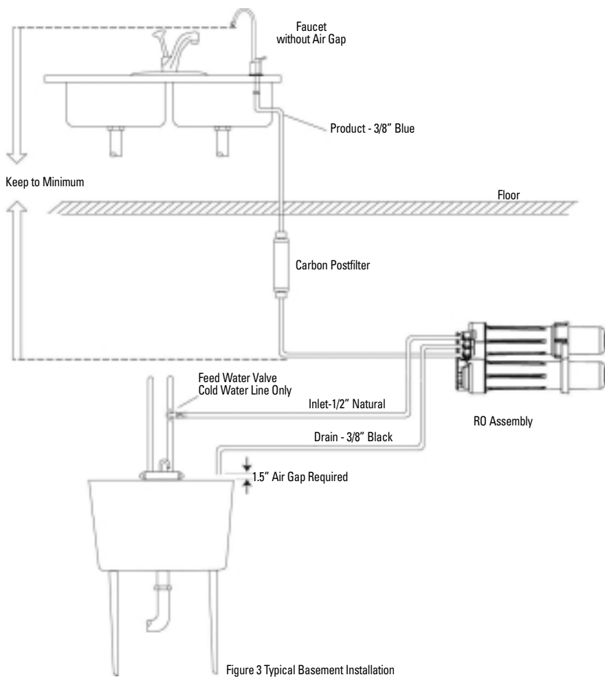
Figure 3 Typical Basement Installation
